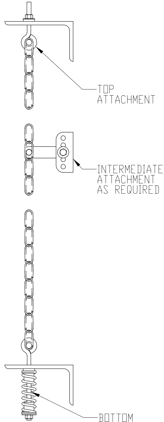
SIDE VIEW
