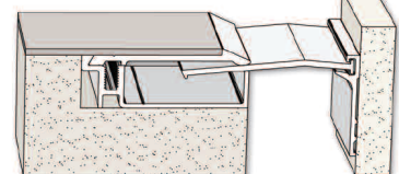
Series HFXREH Floor-to-Wall / New-to-Existing Nominal Joint Openings 1" to 4"
