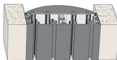
Series VSS-E 700 & Larger Wall-to-Wall / Exterior (shown) / Interior (similar) Nominal Joint Openings 7" to 24"+
