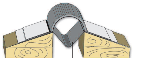
Series ERJ Roof-to-Roof / Low Profile Rubber Bellows Nominal Joint Openings 2" to 6"
