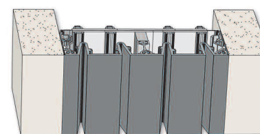
Series VSS-I 700 & Larger Wall-to-Wall / Exterior (shown) / Interior (similar) Nominal Joint Openings 7" to 24"+
