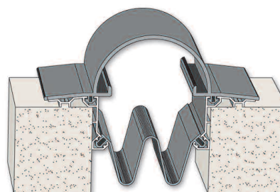
Series RSS Roof-to-Roof / Silicone Bellows Nominal Joint Openings 2" to 10"
