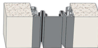
Series VSS-I 200-600 Wall-to-Wall / Interior Nominal Joint Openings 2" to 6"
