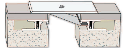
Series LAST Floor-to-Floor / Blockout Mount Nominal Joint Openings 1" to 18" NOTE: Also available as Floor-to-Wall system
