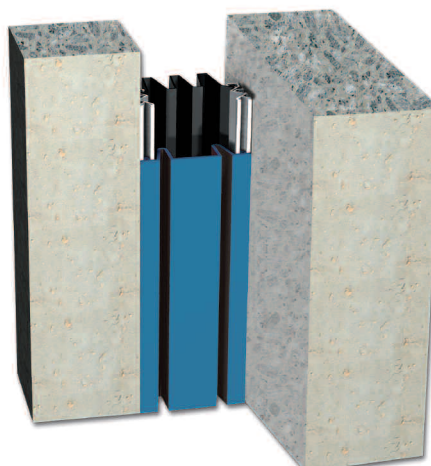
Series VSS-E 700 & Larger Wall-to-Wall / Exterior (shown) / Interior (similar) Nominal Joint Openings 7" to 24"+
