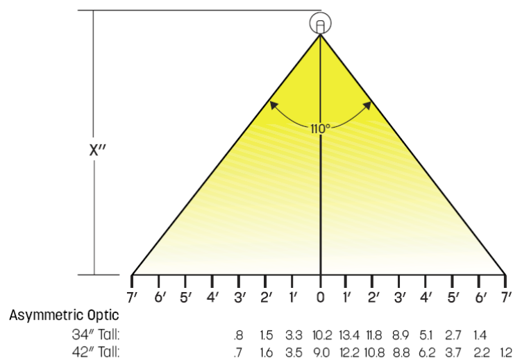
Foot Candle Chart
