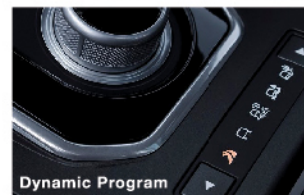
Dynamic Program
